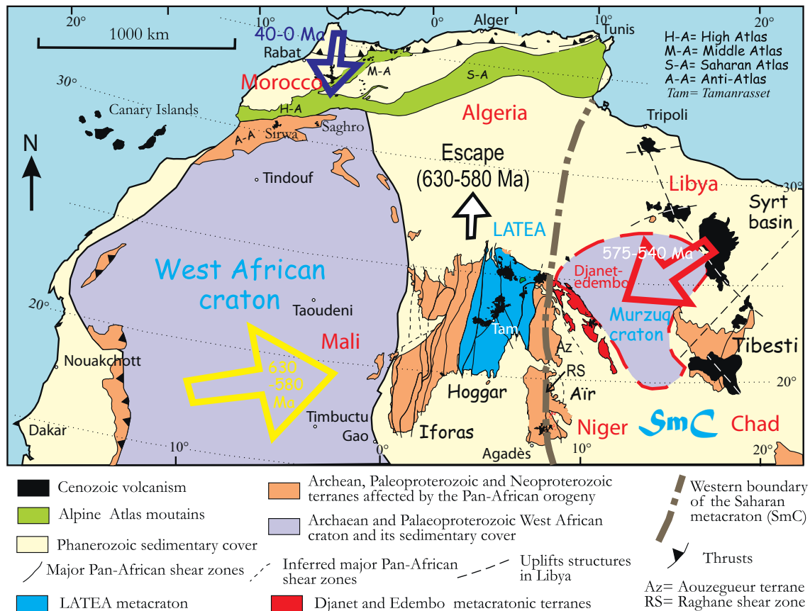
Fig. 10. Main rheological domains from North-West Africa with enhancement of the LATEA metacraton and of the Djanet and Edembo metacratonic terranes (see text). The Cenozoic volcanism is represented showing that it is located within the LATEA metacraton and within the metacratonic area around the Murzuq craton. Adapted from Liégeois et al. (2005) and Fezaa et al. (2010).
