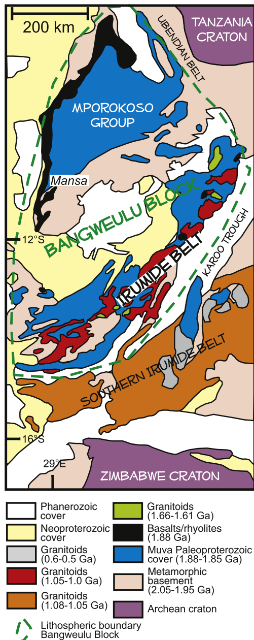
Fig. 8. Geological map of the Bangweulu Block, the Irumide Belt and adjacent areas. Modified from De Waele et al. (2006).
