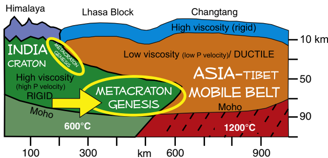
Fig. 4. Section of the lithosphere showing the current relation between the thick, cold and rigid Indian lithosphere and the thin, hot and ductile lithosphere of Tibet. Craton boundaries are submitted to high stress, pressure and temperature that can lead to their partial reactivation without lithospheric thickening, i.e. to their metacratonization, at high and low depth. Adapted from Bendick and Flesch, 2007.
