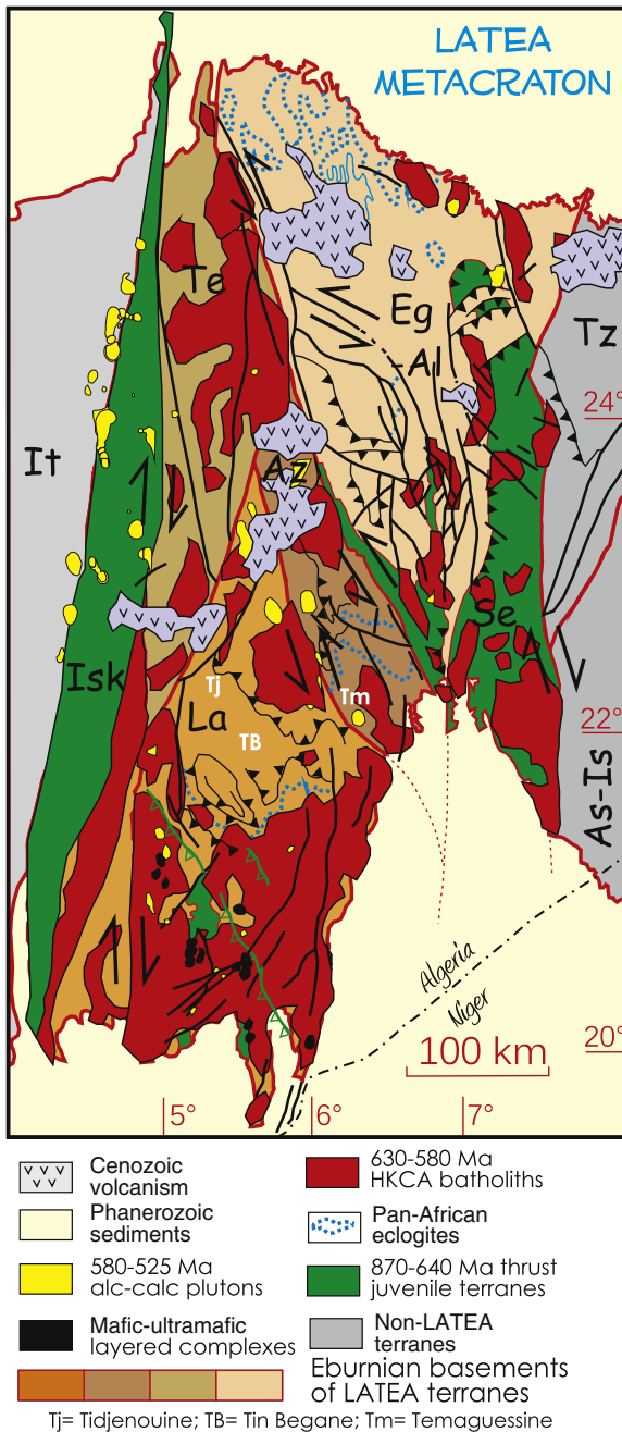
Fig. 11. Geological map of the LATEA metacraton showing the preserved Archean–Paleoproterozoic basement (metacraton) dissected in four terranes (La=Laouini, Az=Azrou-n-Fad, Te=Tefedest, Eg-Al=Egêrê-Aleksod), the thrust juvenile Cryogenian terranes (ISK=Iskel, Se=Serouenout with additional more localized material such as the eclogitic bands), the high-K calc-alkaline (HKCA) batholiths (630–580 Ma), the mantle-derived mafic–ultramafic layered complexes, the alkaline/alkali-calcic plutons (principally Taourirts Province) and the Cenozoic Tuareg volcanism mainly located in the LATEA metacraton. Neighbor terranes are In Tedeini (It), Tazat (Tz) and Assodé-Issalane (As-Is). Adapted from Liégeois et al. (2003).
